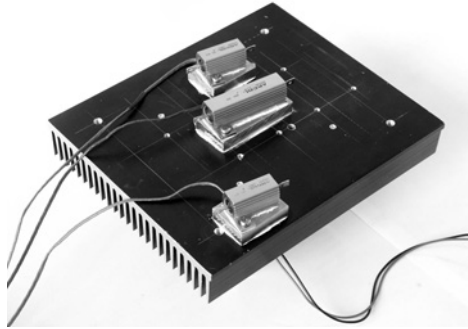
Fig.11: For testing the theory, three different heat sources are mounted onto the heat sink. The heat sources are labeled HSa , HSb , and HSc from the back to the front (see Fig.10). The center point coordinates of these three heat sources are HSa ( -38.5 \text{ mm}/-14 \text{ mm} ), HSb ( 0/0 ) and HSc ( 57.5 \text{ mm}/47 \text{ mm} ). Each heat source consists of a heating resistor on a copper heat spreader of 8 \text{ mm} thickness containing a 1.5 \text{ mm} diameter hole with inserted thermocouple. HSa and HSc (both emitting 55 \text{ W} thermal power) have a 33 \times 25 \text{ mm}^2 heat spreader area, HSb ( 75 \text{ W} ) has a heat spreader area of 53 \times 25 \text{ mm}^2 . Note that the coordinate system employed here and also shown in Fig.10 is different to the coordinate system of Fig.1(a) that has to be employed if (2) – (9) are used.
