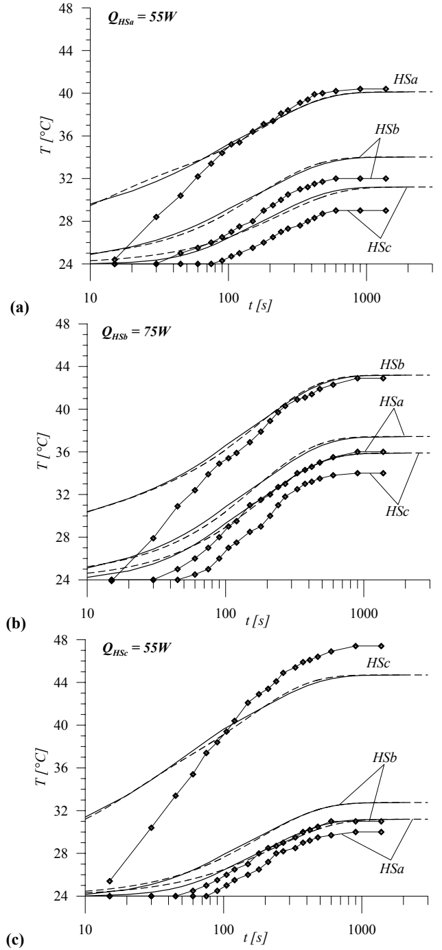
Fig.12: Thermal step responses of all three heat sources HSa , HSb and HSc for heating (a) only HSa with Q=55 \text{ W} , (b) only HSb with Q=75 \text{ W} and (c) only HSc with Q=55 \text{ W} . The dots are experimentally measured, and the solid lines are resulting from the transient FEM simulation of the simplified heat sink model. The dashed lines are resulting from the RC thermal equivalent network model as described in section 4 and in the Appendix.
