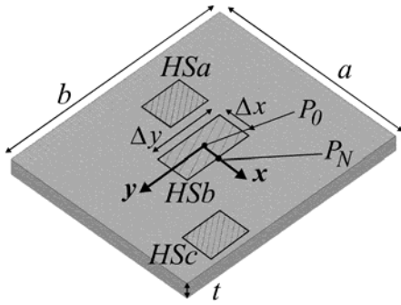
Fig.10: Simplified thermal heat sink model of the extruded heat sink (Fig.9) with h=220 \text{ W/m}^2\text{K} , t=12.7 \text{ mm} , a=150 \text{ mm} , b=177 \text{ mm} , k=205 \text{ W/mK} . The 2D heat sources are sized and located as described in Fig.11.
