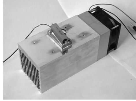
Fig.5: Hollow-fin cooling aggregate ( 150 \times 80 \times 80 mm^3 , 10.5mm base plate thickness, aluminium with k=205W/mK ) with fan. A test heat source of Q=100W is mounted onto the center. The shown wire is connected to a thermocouple inserted in the copper-heat spreader below the heating resistor to measure the center point temperature ( P_0 in Fig.1). The heating resistor is not connected to a voltage source yet.
