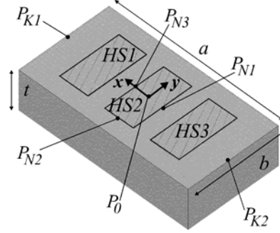
Fig.6: Simplified thermal heat sink model of the hollow-fin cooling aggregate (Fig.5) according to Fig.1(b) with h=650W/m^2K and t=36mm , a=150mm , b=80mm , k=205W/mK . In the FEM simulation the bottom wall is defined employing a Neumann boundary condition with h=650W/m^2K=const , all other walls are defined as thermally isolating. The heat sources are modeled as 2D-elements with continuous heat distribution.
