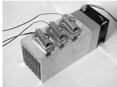
Fig.7: For testing the theory, three 100W -heat sources are mounted onto the heat sink. Each heat source consists of a heating resistor on a 25 \times 53mm^2 copper heat spreader of 8mm thickness containing a 1.5mm diameter hole with an inserted thermocouple for temperature measurement. The heat sources are labeled HS1 , HS2 , and HS3 from the left to the right (opposite direction of the airflow, see also Fig.6). The space between two neighbor heat sources is 15mm .
