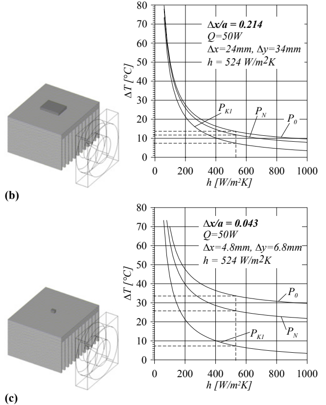
Fig.3: Centered test heat sources of different size (characterized by \Delta x/a -ratio) result in different temperature measurements at selected points P_0 , P_N , P_{KI} on the heat sink with a = 112 \text{ mm} , b = 100 \text{ mm} , t = 10 \text{ mm} , k = 205 \text{ W/mK} (see Fig.1(b)). The heat transfer coefficient h describes only the convection cooling of the heat sink via the fins and is, therefore, not affected by the test heat source geometry.
