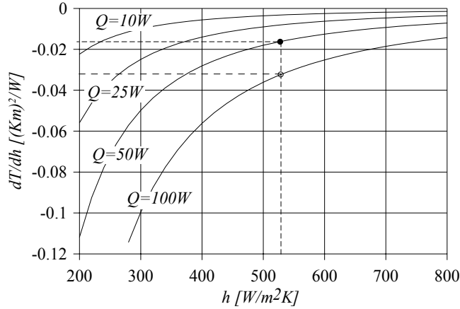
Fig.4: The derivative dT/dh of the heat sink surface temperature dependent on the heat transfer coefficient h and the heating power Q [W]. These curves are independent from \Delta x/a -ratios of the test heat source and also independent from the heat sink surface point of the stationary measurement. The curve of dT/dh for Q=50W shown here is valid for all curves of Fig.3.
