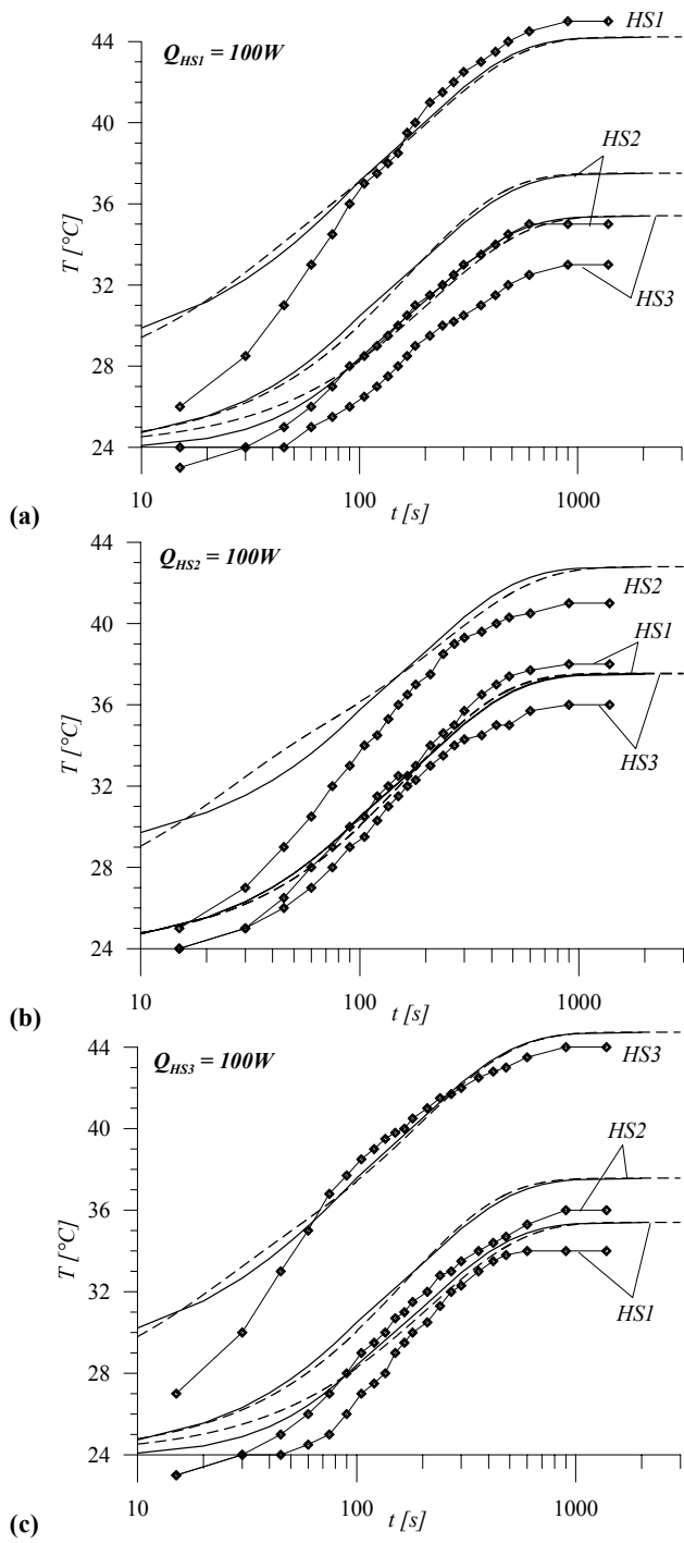
Fig.8: Thermal step responses of all three heat sources HS1 , HS2 and HS3 for heating (a) only HS1 with Q=100W , (b) only HS2 with Q=100W and (c) only HS3 with Q=100W . The connected dots are experimentally measured, the solid lines are resulting from transient FEM simulations of the simplified heat sink model. The dashed lines are resulting from the RC thermal equivalent network model as described in section 4 and in the Appendix.
