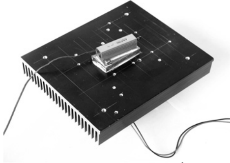
Fig.9: Extruded heat sink ( 150 \times 177 \times 26.5 \text{ mm}^3 , 5 \text{ mm} base plate thickness, aluminium with k=205 \text{ W/Km} ) with a fan mounted onto the bottom side (only the wires of the fan are visible in the photo). A test heat source of Q=100 \text{ W} is mounted onto the center. The shown wire is connected to a thermocouple inserted in the copper-heat spreader below the heating resistor to measure the center point temperature ( P_0 in Fig.6).
