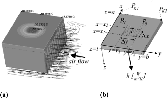
Fig.1: (a) A CFD simulation shows the temperature field and air flow for a heat sink. In the vicinity of the power module there is a hot spot. (b) The simplified heat sink model consists of a plate with a heat transfer coefficient h=const as boundary condition at the bottom side, and thermal isolation ( h=0 ) at all other surfaces.
