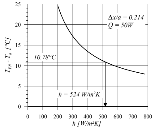
Fig.2: Dependency of the temperature at surface point P_N on the heat transfer coefficient h [ W/m^2K ] for an air-cooled heat sink ( a=112mm , b=100mm , t=10.5mm ) with a power module of \Delta x=24mm ( \Delta x/a=0.214 ), \Delta y=34mm and Q=50W . The curve is derived analytically from (2) – (9) and/or (10). The thermal conductivity of the extruded aluminium heat sink is k=205 W/mK . The temperature \Delta T=T_{PN}-T_a=10.78^\circ C is derived from a stationary CFD-simulation (by ICEPAK) of the heat sink shown in Fig.1.
