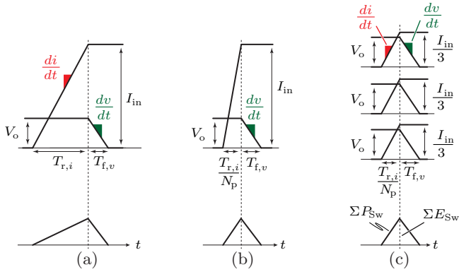
Fig. 2.11: Comparison of switching losses between a single boost converter (a) and parallel-interleaved boost converters (c) for the same rates of dv/dt and di/dt . The single boost converter can only reach the same level of switching losses as the parallel-interleaved converter, if the rate of di/dt is increased by a factor of N_p (b).
