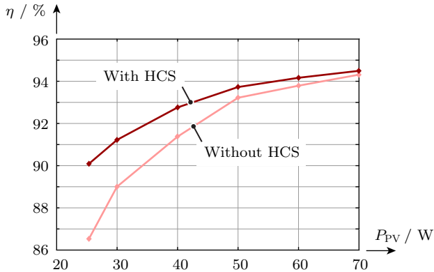
Fig. 3.27: Comparison between the measured efficiency of the prototype in half-cycle skipping (HCS) mode and in normal HC-DCM for an input voltage of V_{PV} = 35 \text{ V} at low levels of converter input power P_{PV} .
