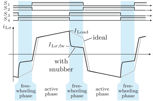
Fig. 4.13: Effect of a large snubber capacitor on the freewheeling current of the transformer leakage inductance.
