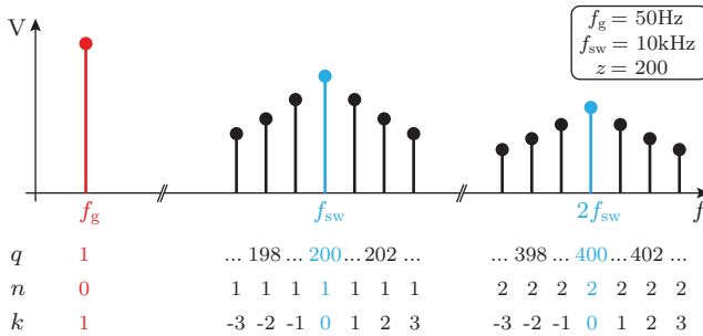
Fig. 4.4: Explanation of the nomenclature used to specify the order q = n \cdot z + k of the harmonics with the example of f_g = 50 \text{ Hz} and f_{\text{sw}} = 10 \text{ kHz} .
