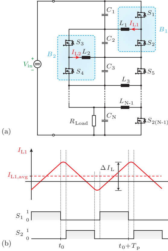
Fig. 5.3: New Rainstick converter (RSTC) topology: (a) circuit diagram showing a capacitive voltage divider ( C_1 \dots C_N ) and balancing modules ( B_1, B_2 , highlighted) and (b) inductor current waveform and gate signals of one balancing module.
