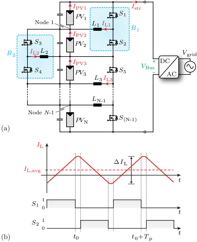
Fig. 3.29: Analyzed PV system with balancing circuits: (a) circuit diagram showing a PV string with N PV panels ( PV_1, \dots, PV_N ), N-1 balancing converters ( B_1, \dots, B_{N-1} ) and a grid connected DC/AC converter and (b) characteristic inductor current waveform and gate signals of one balancing converter.
