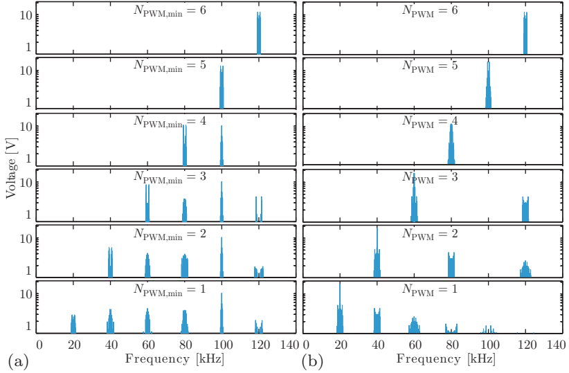
Fig. 4.22: Comparison of the harmonic spectrum of the input voltage v_{\text{FB,tot}} of the series connection of AC/DC converter cells (without the 50 Hz low-frequency component) for different 4D-interleaving schemes: (a) variable number of PWM modules ( N_{\text{PWM,min}} denotes the minimum number of active PWM modules); (b) fixed numbers of PWM modules N_{\text{PWM}} where the remaining cells are operated as fundamental frequency modules. (System with 6 cells and a switching frequency of the PWM cells of f_{\text{sw,PWM}} = 20 \text{ kHz} and a DC-link voltage of each cell of V_{\text{DC,cell}} = 66 \text{ V} .)
