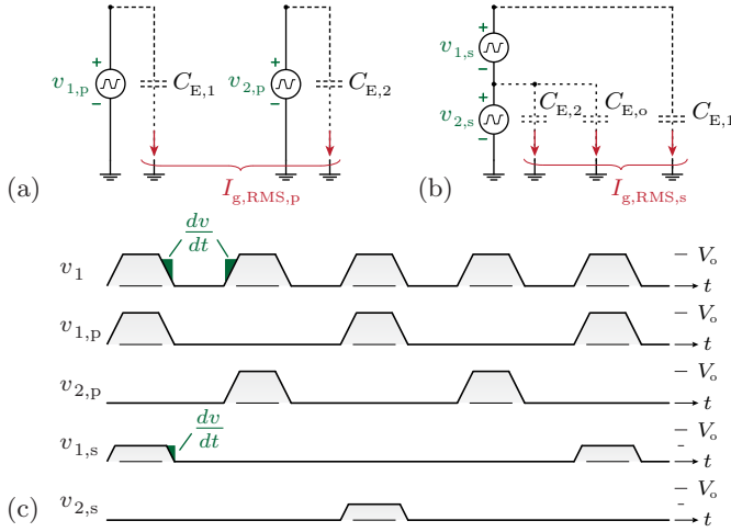
Fig. 2.12: Equivalent circuit models for ground currents of (a) the parallel-interleaved boost converter and (b) the series-interleaved boost converter. The waveforms of the switch-node voltages of the parallel-interleaved system ( v_{1,p} , v_{2,p} ) and series-interleaved system ( v_{1,s} , v_{2,s} ) are compared to those of a single boost converter ( v_1 ) in (c) under the assumption of same dv/dt in all systems.
