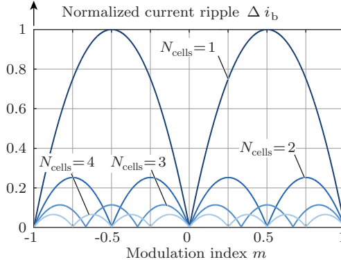
Fig. 4.3: Peak-to-peak current ripple reduction of the boost inductor current i_b (normalized to V_{DC}/(4f_{sw}L_b) ) for different numbers of rectifier stages N_{cells} in dependency of the modulation index m = v_{FB,tot}/V_{DC} for a given value of boost inductance L_b .
