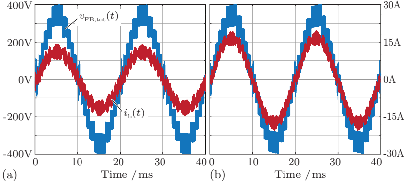
Fig. 4.15: Measured waveforms of the operation of the AC/DC stages of the multi-cell telecom rectifier with a grid voltage of V_{g,RMS} = 230 V: (a) measurement of the converter input voltage v_{FB,tot} and the boost inductor current i_b for a load power of P_L = 1.5 kW and (b) for a load power of P_L = 2.5 kW.
